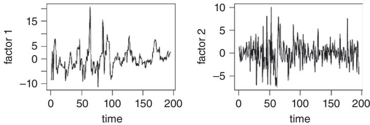
Figure 10.A.1 The two factors used in factor modeling for the first component Z_{1,t} GDP252.
