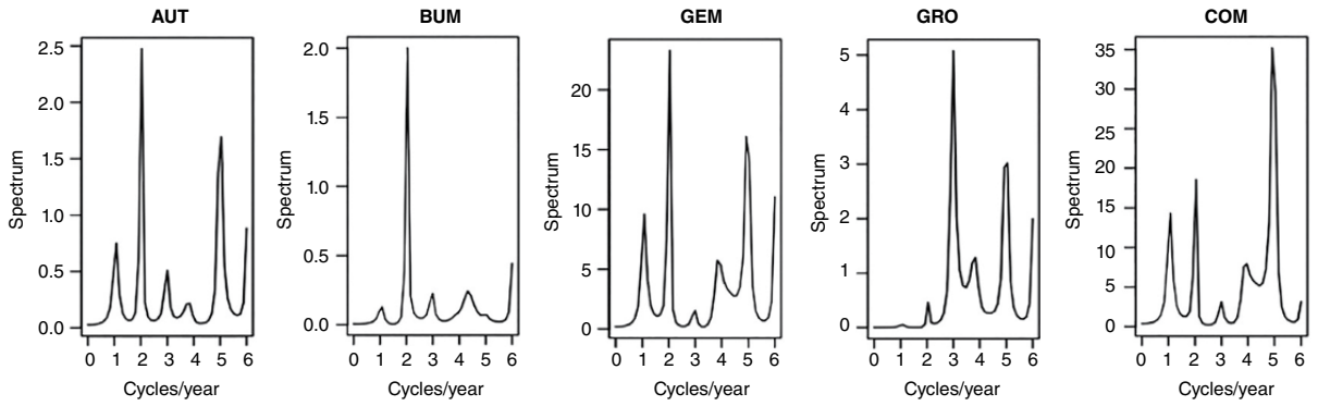
Figure 9.8 The estimated power spectra by using the VAR(4) model.
