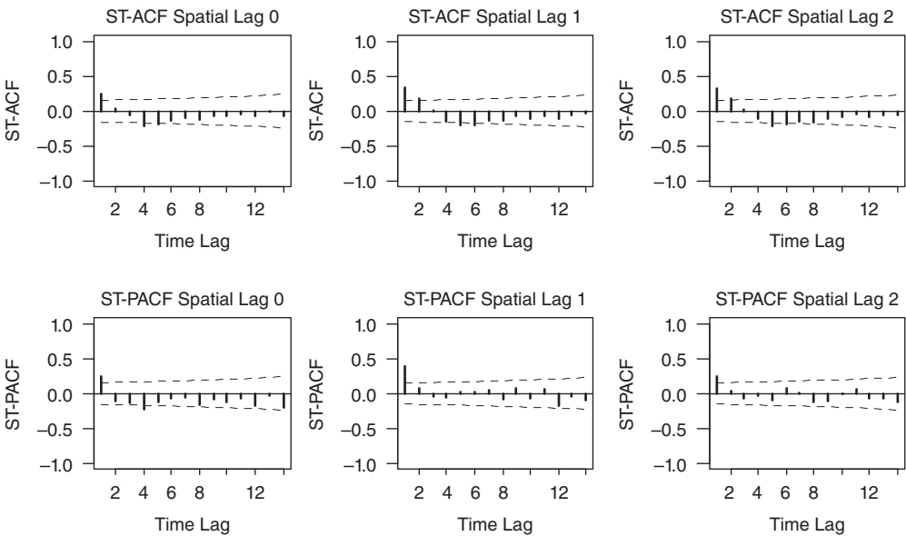
Figure 8.9 The sample ST-ACFs and ST-PACFs for the series \mathbf{Z}_t .
