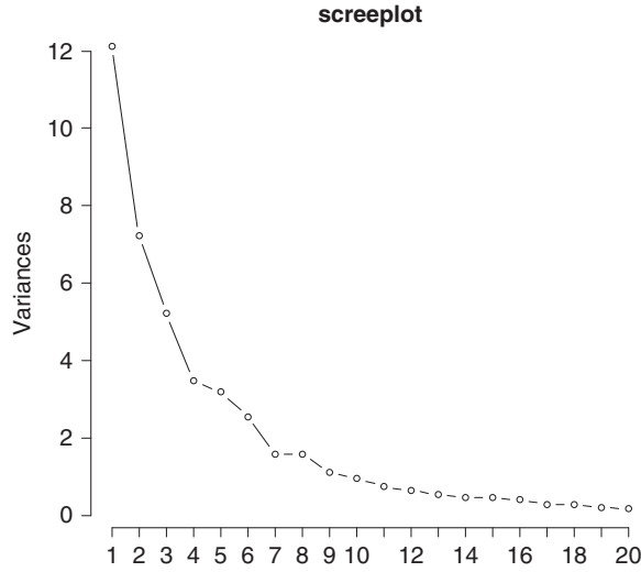
Figure 5.5 The screeplot for standardized variables.
