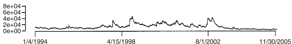
Figure 6.4 The estimated volatilities of the S&P 500 daily log-return between January 4, 1994 and December 30, 2005.
