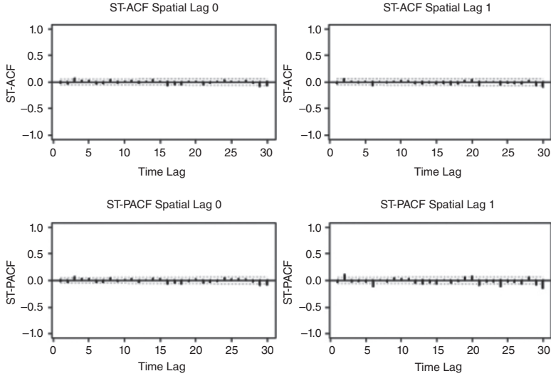
Figure 8.7 The sample ST-ACFs and ST-PACFs of the residuals from the fitted STAR (2_{1,0}) \times (2_{0,1})_{12} model.
