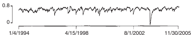
Figure 6.5 The estimated conditional correlation between the returns of S&P 500 and BAC from January 4, 1994 to December 30, 2005.
