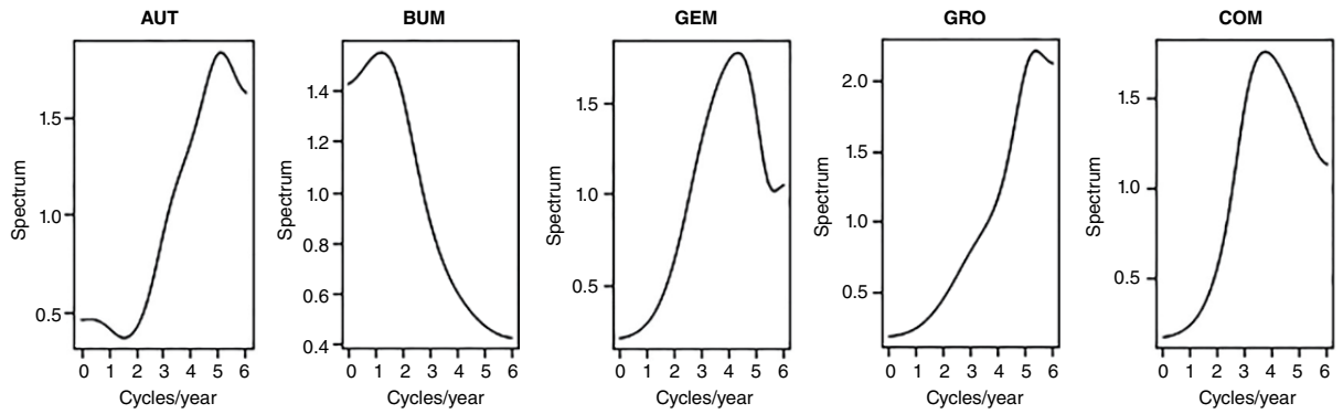
Figure 9.7 The estimated spectra by the penalized Whittle likelihood method of Krafty and Collinge (2013).
