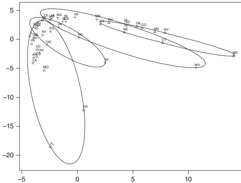
Figure 10.11 PAM cluster plot of the STD data set.
