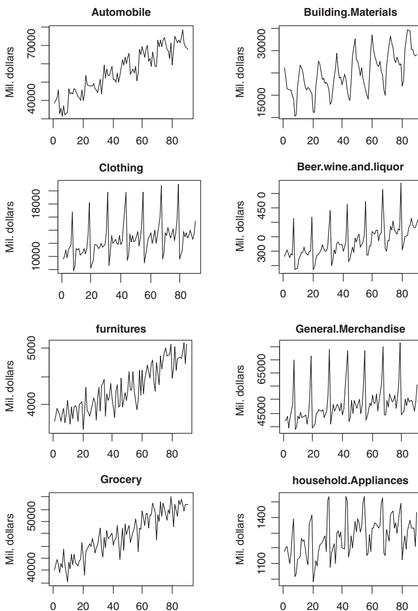
Figure 2.1 US monthly retail sales revenue from June 2009 to November 2016.
